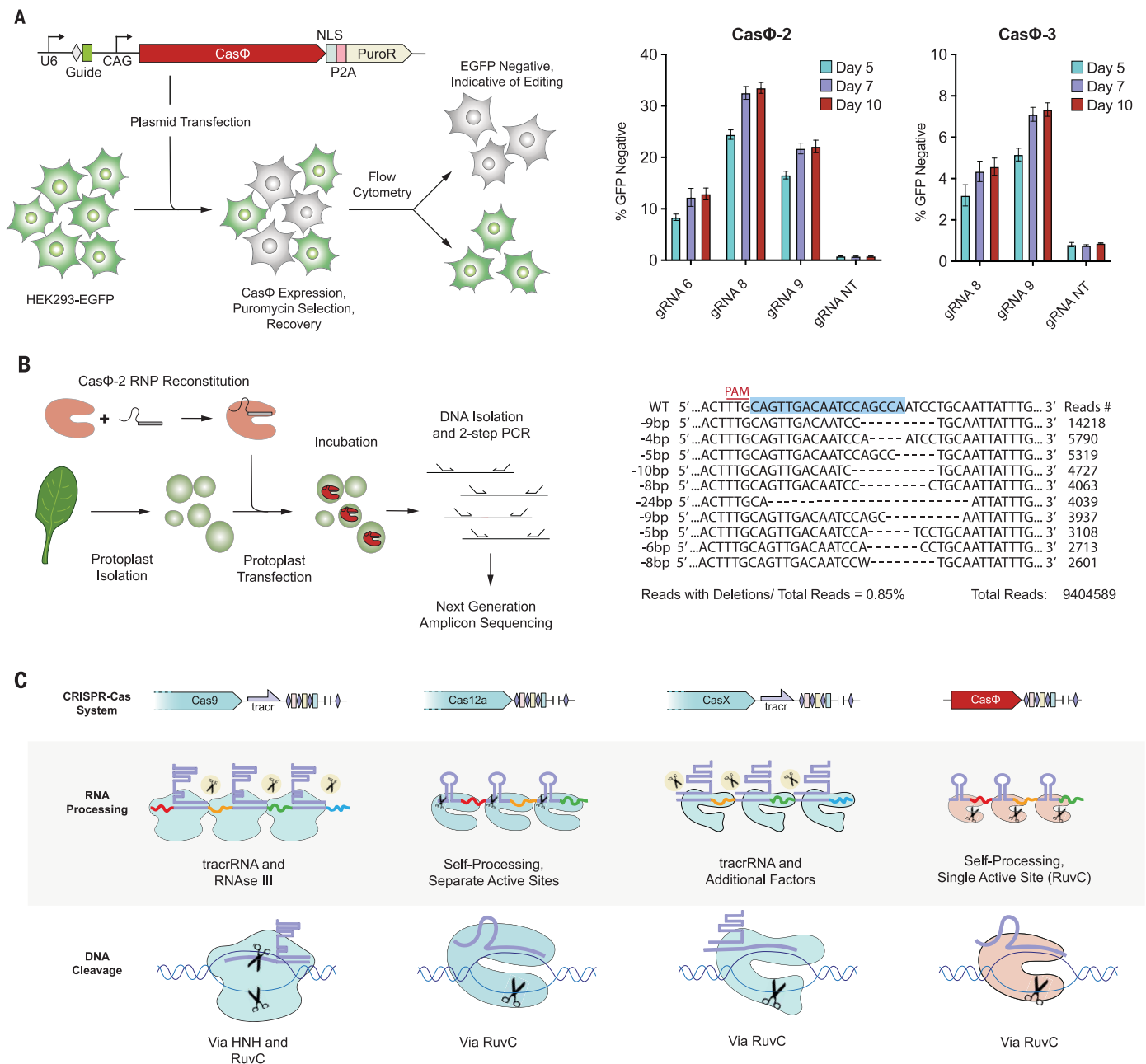
Fig. 4. Cas \Phi is functional for genome editing. (A) Experimental workflow of the GFP disruption assay (left) and GFP disruption using Cas \Phi -2 and Cas \Phi -3 and a nontargeting (NT) guide as a negative control ( n = 3 each; means \pm SD). (B) (Left) Experimental workflow of Cas \Phi 2 RNP-mediated genome editing in A. thaliana mesophyll protoplasts. (Right) Amplicon sequencing data showing the most frequent deletions for gRNA33 in the targeted region (blue) within the AtPDS3 gene. (C) Scheme illustrating the differences in RNA processing and DNA cutting for Cas9, Cas12a, CasX, and Cas \Phi .
